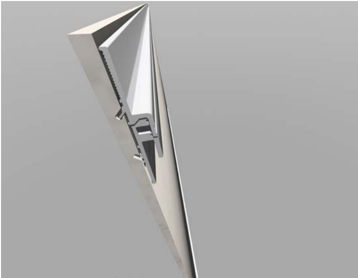
Image 44: Neolith slab with the Strongfix System profiles
