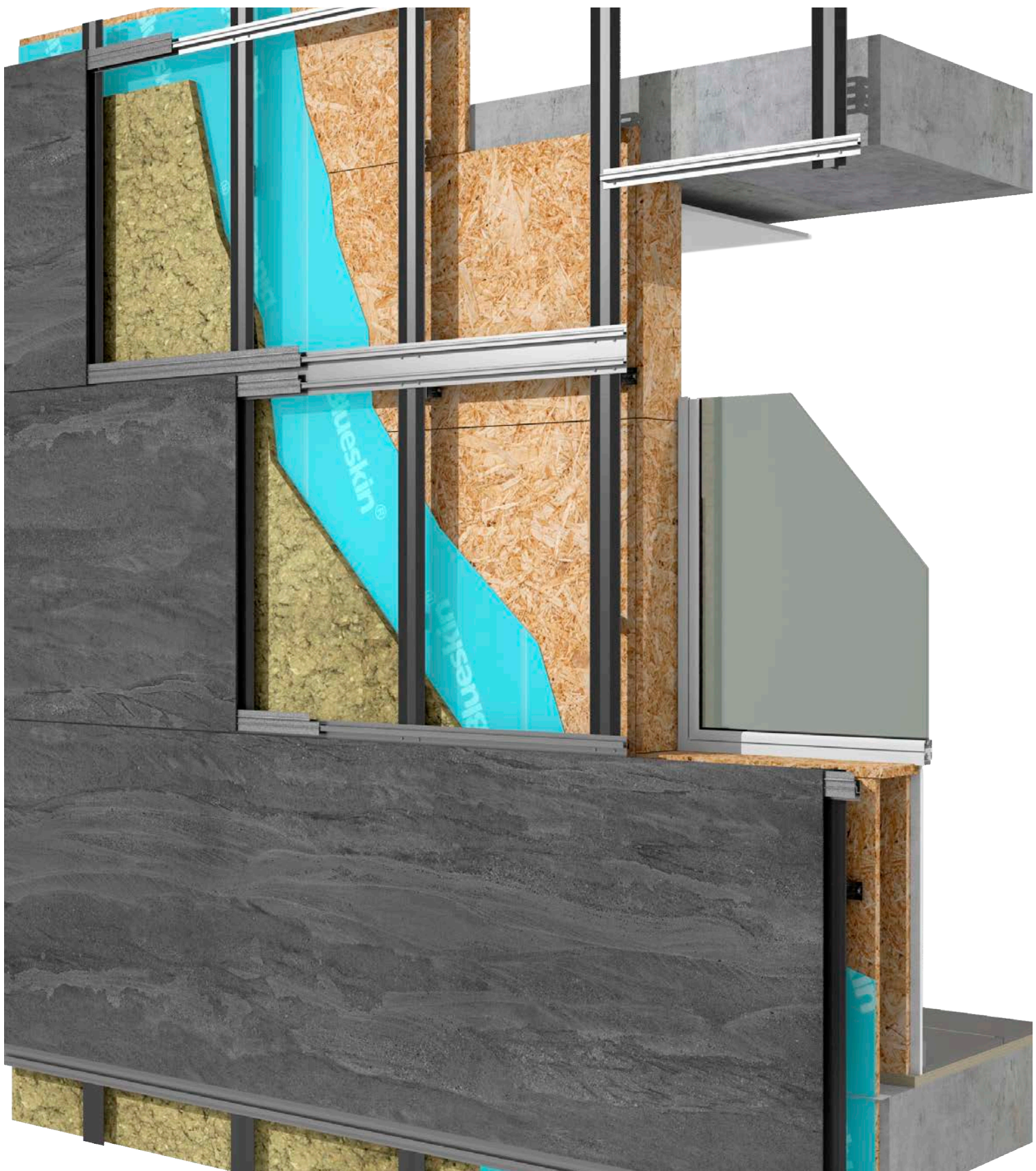
Image 37: Strongfix System mockup
