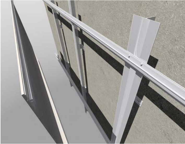
Image 42: Strongfix System installation Step 2
