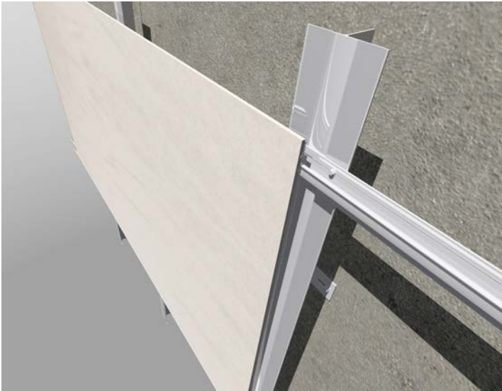
Image 43: Strongfix System installation Step 3
