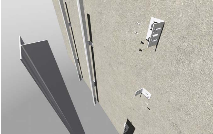
Image 19: HC System installation Step 1
