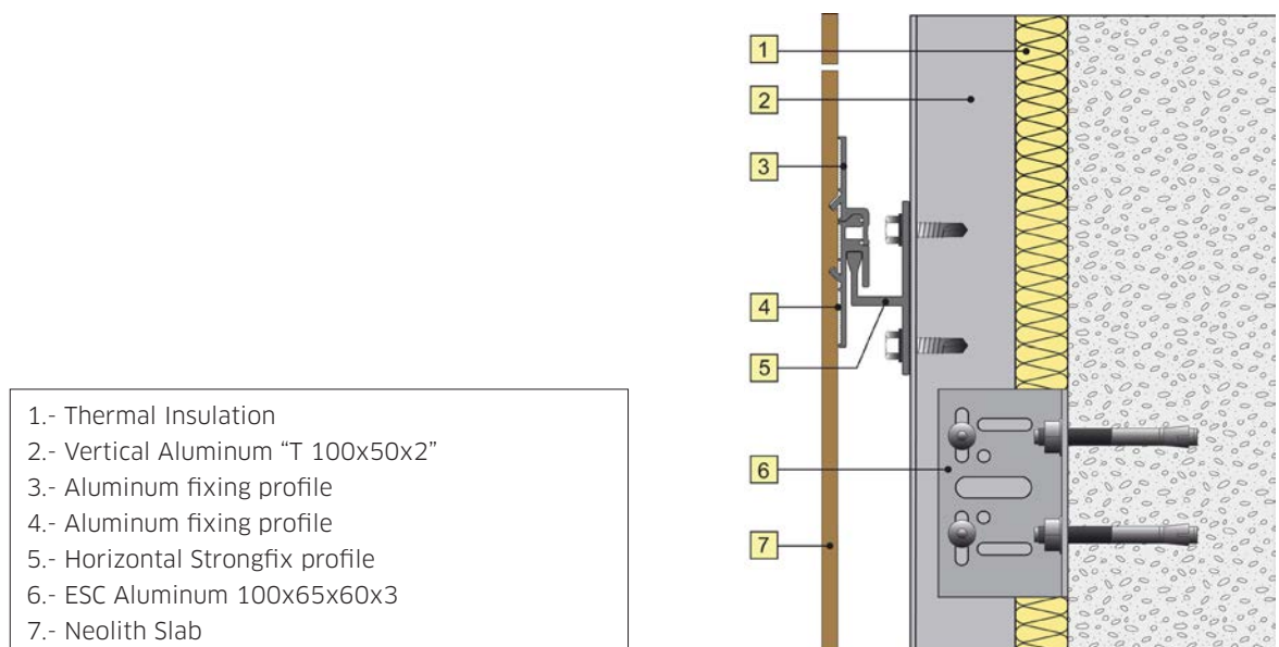
Image 38: Strongfix System vertical section
