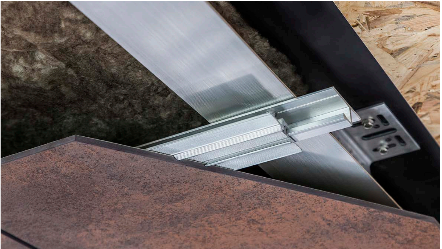
Image 39: Strongfix System detail
