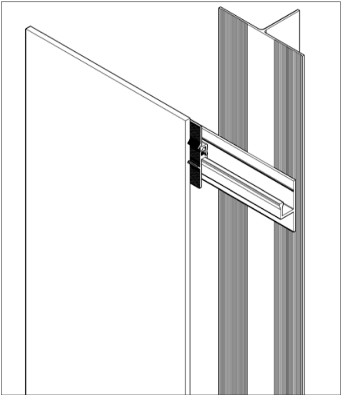
Image 48: Strongfix System detail
